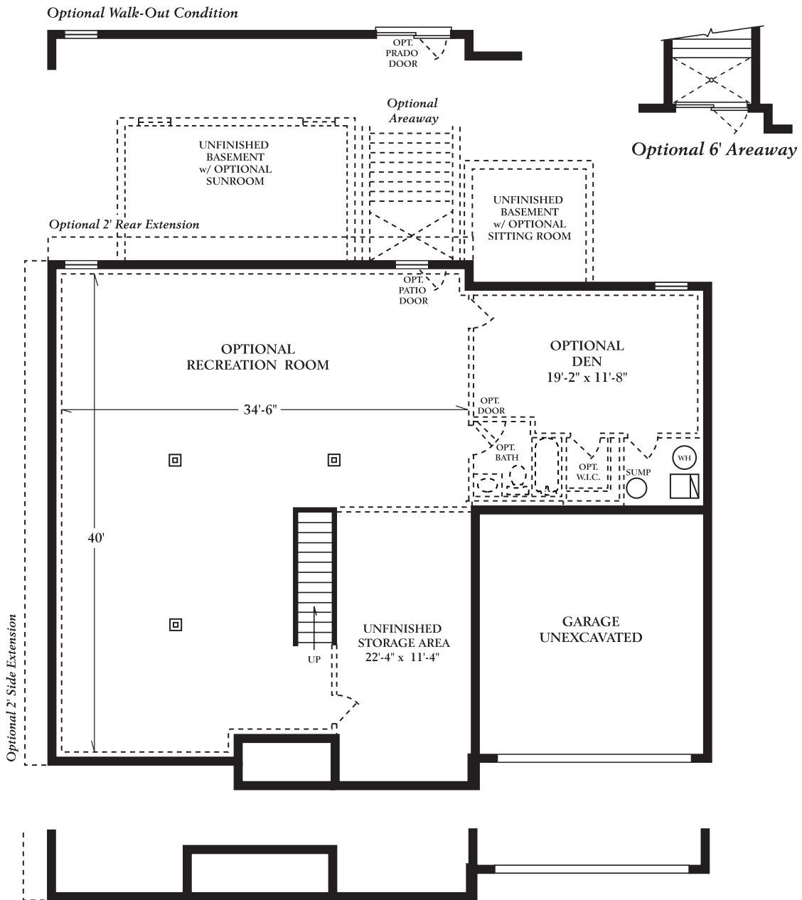
Partial Basement Plan for Elevation #3
